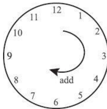
Diagram 8.2: Clock Arithmetic
