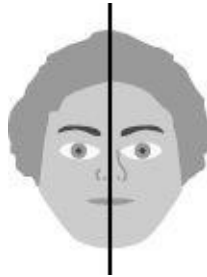
Fig. 11.1: Symmetric Face
