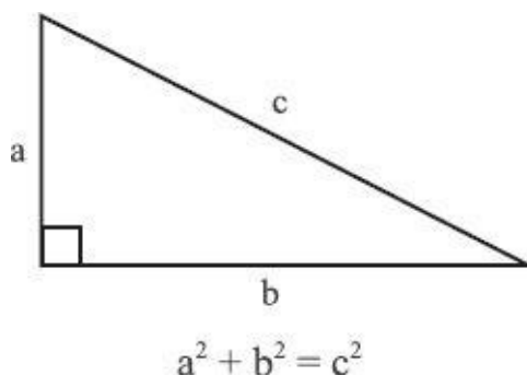
Diagram 15.1: Pythagorean Theorem
