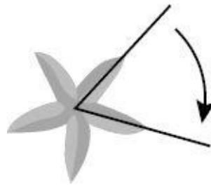
Fig. 11.2: Symmetric Starfish
