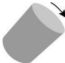
Fig. 11.3: Symmetric Cylinder
